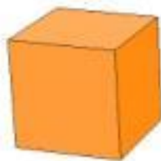
hexahedron zesvlak
